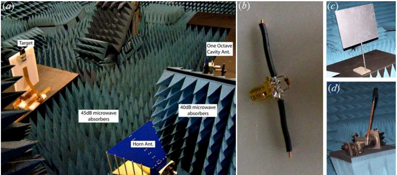
Fig. 9. (a) The general experimental layout, and the targets: (b) a BAT54 Schottky diode (dipole+diode target); (c) a piece of 34 \times 40 \text{ cm}^2 aluminium plate mounted on an iron stand; and (d) a rusty bench clamp. One of the mobile phones can be seen in the target position in panel (a).
