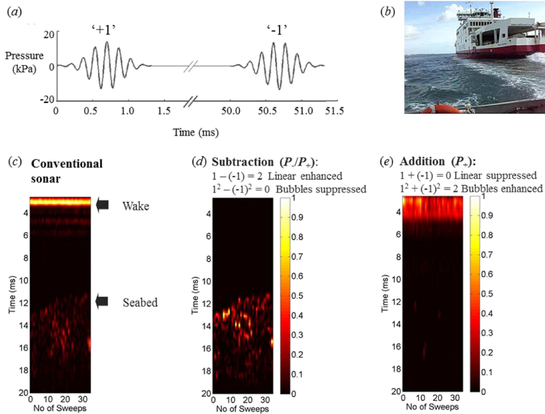
Fig. 4. (a) The two sonar pulses used in this particular test, as measured 2.6 m in front of the sonar in clear water in a test tank. The 50 ms interval between pulses is chosen to be sufficiently short that the environment (especially the bubbly wake) has not evolved too much between the two pulses as to make TWIPS inoperable, but long enough to mean that, for ranges up to around 37.5 m, only one pulse is in the water at once, avoiding range ambiguities. (b) Photograph of the stern of the MV Red Osprey as the vessel containing the TWIPS sonar entered its wake, moments before the data of panels (c)–(e) were taken. In panels (c)–(d), the same set of data is processed three ways. Pairs of TWIPS pulses are emitted with 1 s between the start of each pair, and the number of the pair is recorded on the horizontal axis. The two-way time of flight (a proxy for the range) is given on the vertical axis. The panels show the result of processing (c) in a conventional sonar manner, (d) using the P_-/P_+ TWIPS function, and (e) using the P_+ TWIPS function. For details on the processing and the colour scale, see LEIGHTON et al. (2010).
