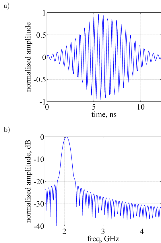
Fig. 8. (a) Time history of one pulse in the pair, showing the normalised amplitude of the Gaussian-modulated waveform used. (b) The normalised amplitude (in dB) of the waveform used in frequency domain. The measured power referenced to 1 mW measured at 1 m is 35 dB m.
