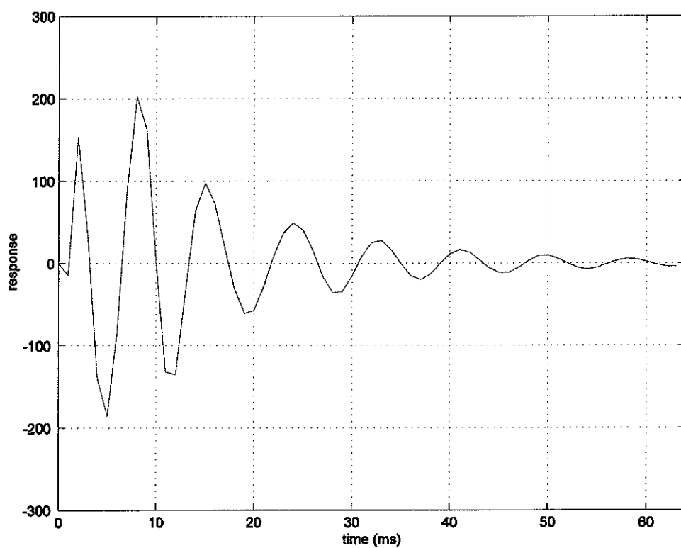
• Figure 48 impulse response from loudspeaker 2 microphone 2
