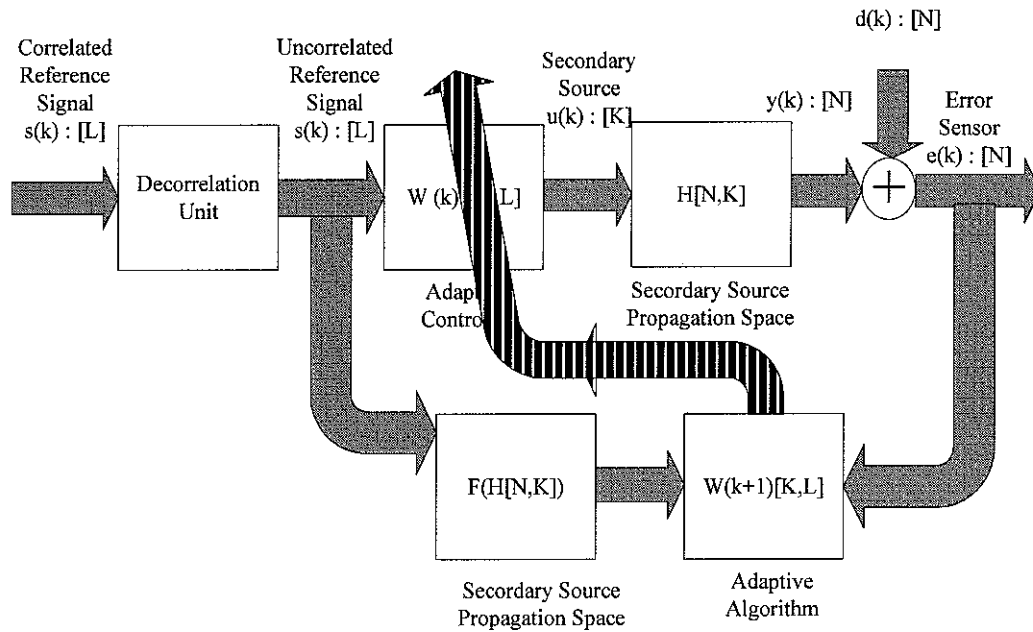
• Figure 45 Block diagram of feedforward ANC system with decorrelatoin unit
