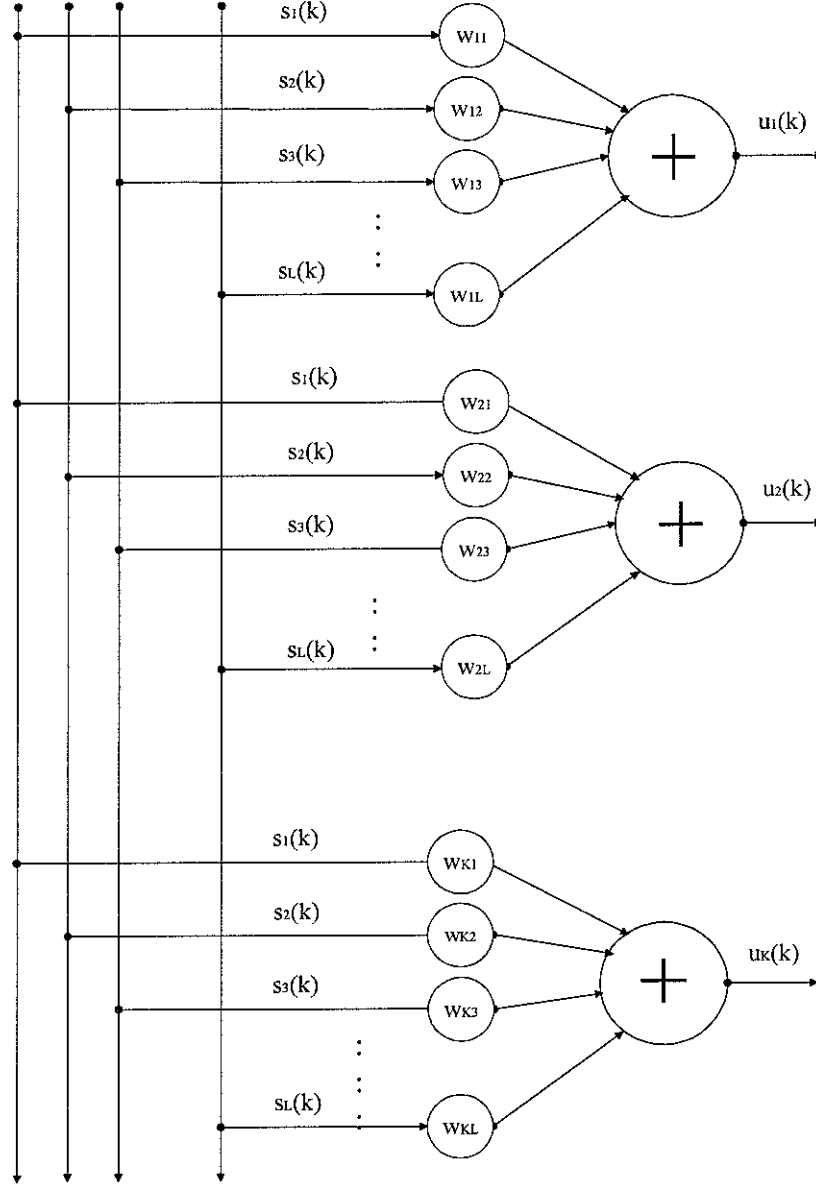
• Figure 42 Diagram of multiple input multiple output adaptive linear combiner
