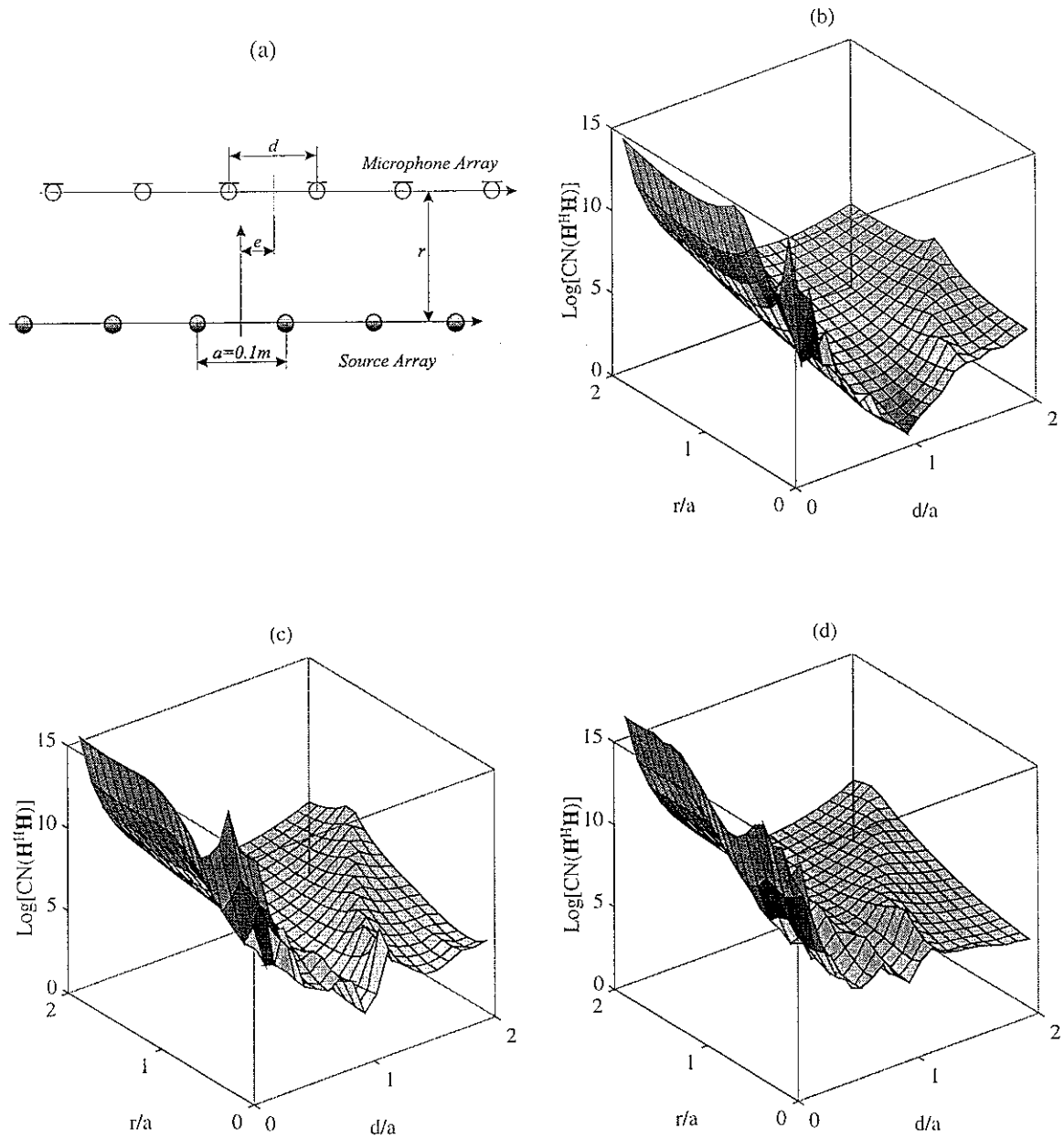
Fig.8 (a) A geometrical arrangement of 6 sources and 6 microphones. Variation of the condition number CN(\mathbf{H}^H \mathbf{H}) with r/a and d/a : (b) ka=0.549 ( =300\text{Hz} ), e=0 , (c) ka=0.549 ( =300\text{Hz} ), e=-0.05m , (d) ka=0.549 ( =300\text{Hz} ), e=0.08m .
