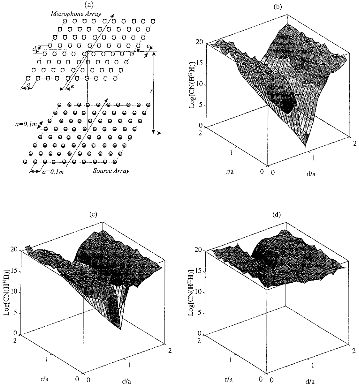
Fig.11 (a) A geometrical arrangement of 100 sources and 100 microphones. Variation of the condition number CN(H^H H) with r/a and d/a : (b) ka=0.549 ( =300\text{Hz} ), e=0 , (c) ka=0.549 ( =300\text{Hz} ), e=-0.05m , (d) ka=0.549 ( =300\text{Hz} ), e=0.08m .
