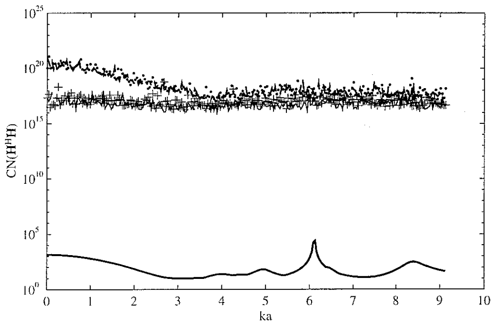
Fig.16 A comparison of condition numbers obtained from the use of five different types of microphone array in measuring the acoustic field generated from the x source array: point represents the condition number obtained by the use of microphones of the horizontal line array, broken line the vertical line array, plus the cross array, thick solid line the X array and thin solid line the square array.
