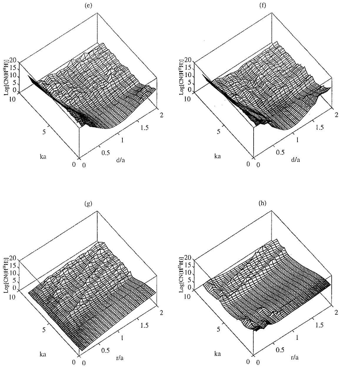
Fig.10 contd Variation of the condition number CN(H^H H) with d/a and ka : (e) r/a=1 , e=0 , (f) r/a=0.5 , e=0 , (g) d/a=1 , e=0 , (h) d/a=0.5 , e=0 .
