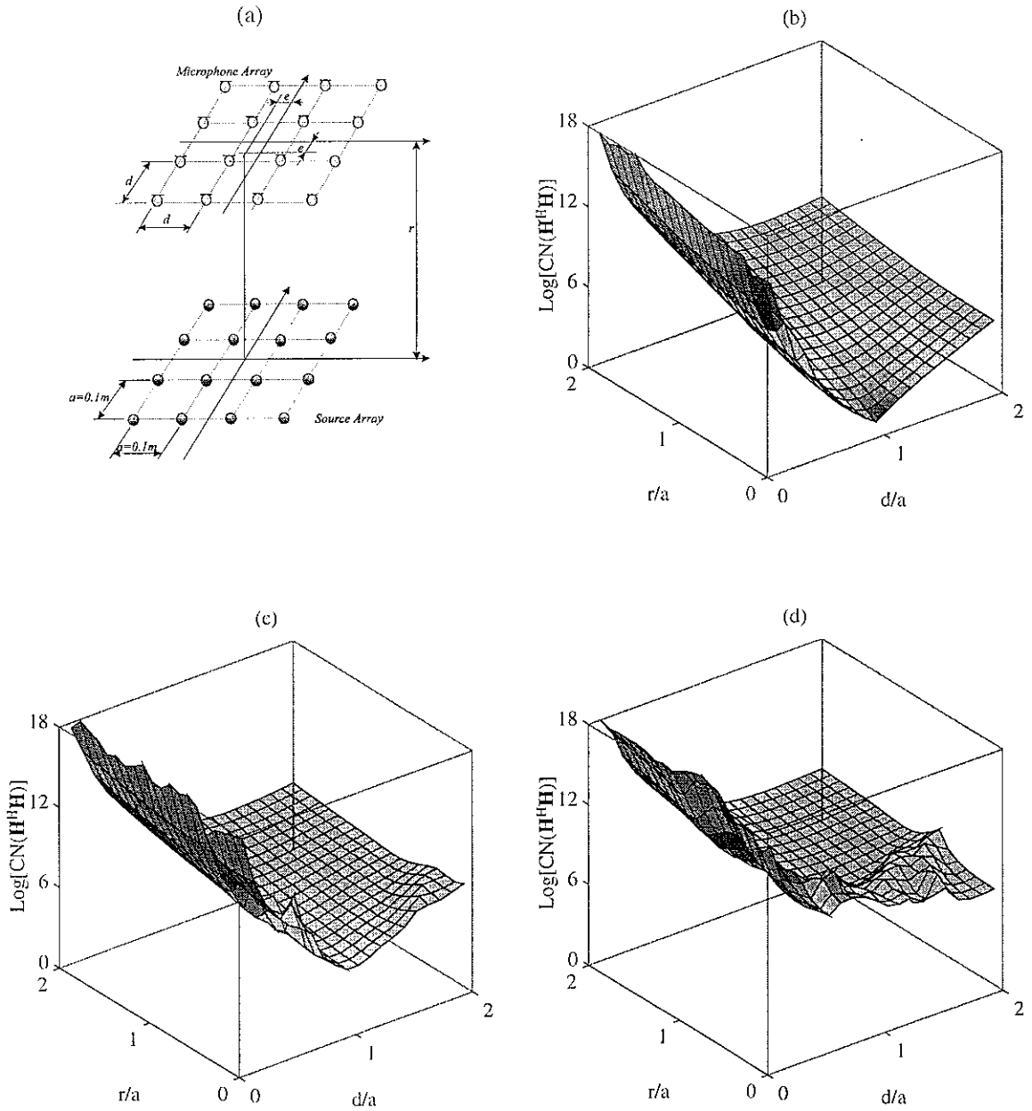
Fig.9 (a) A geometrical arrangement of 16 sources and 16 microphones. Variation of the condition number \text{CN}(\mathbf{H}^H \mathbf{H}) with r/a and d/a : (b) ka=0.549 ( =300\text{Hz} ), e=0 , (c) ka=0.549 ( =300\text{Hz} ), e=-0.05\text{m} , (d) ka=0.549 ( =300\text{Hz} ), e=0.08\text{m} .
