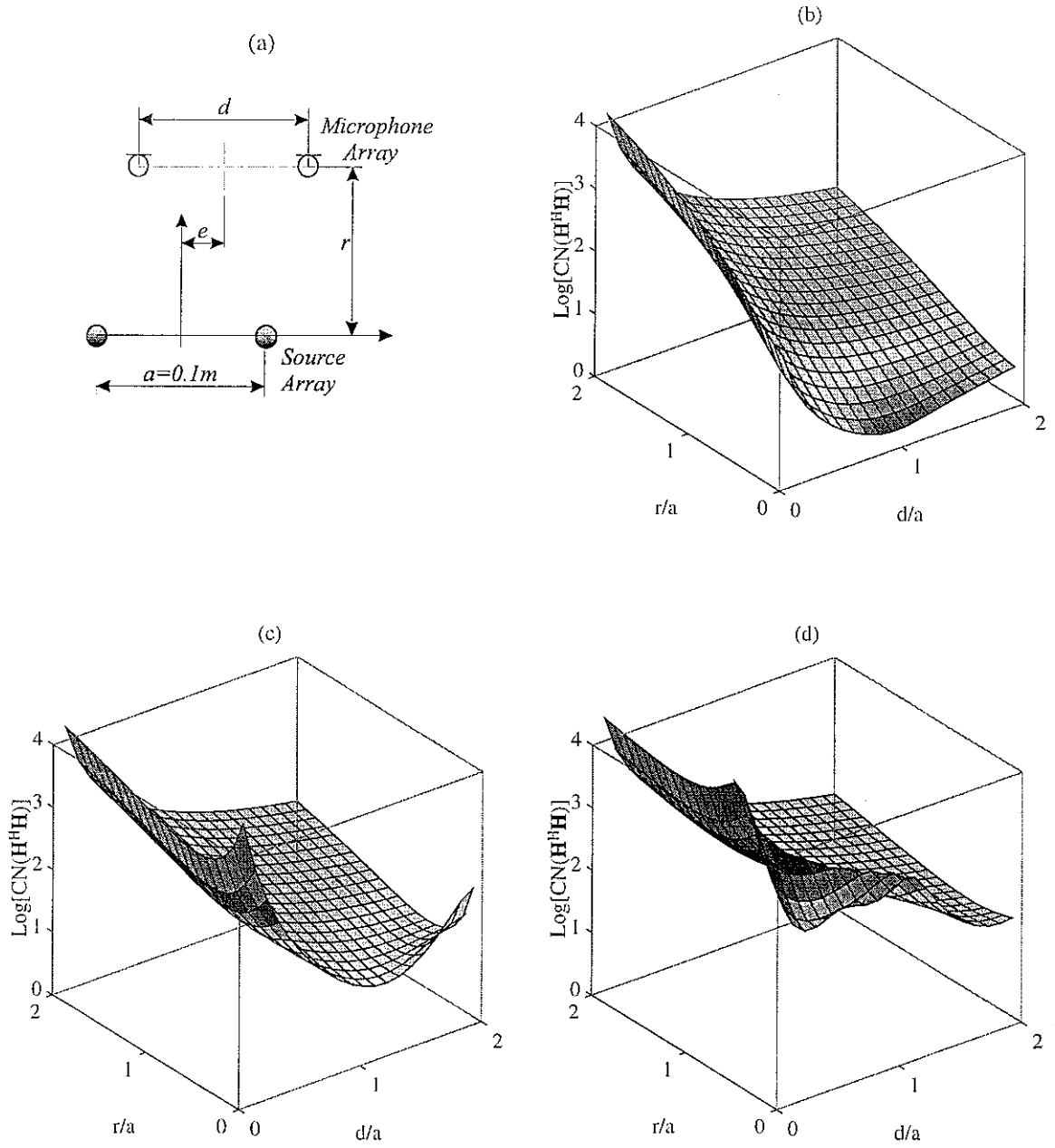
Fig.6 (a) A geometrical arrangement of 2 sources and 2 microphones. Variation of the condition number CN(\mathbf{H}^H \mathbf{H}) with r/a and d/a : (b) ka=0.549 ( \approx 300\text{Hz} ), e=0 , (c) ka=0.549 ( \approx 300\text{Hz} ), e=-0.05m , (d) ka=0.549 ( \approx 300\text{Hz} ), e=0.08m .
