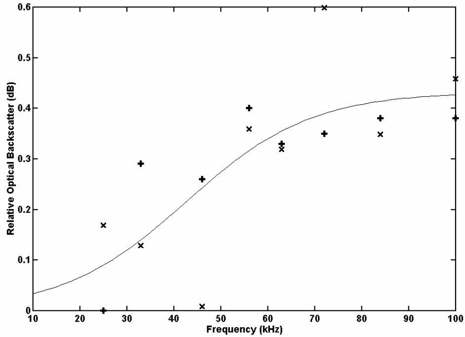
Figure 11 Two sets of data (+, x) showing back-scattered optical power in decibels as a function of the acoustic excitation frequency. The values were calculated relative to the back-scattered optical power in the case when there was no acoustic excitation. A best-fit curve for the combined data sets is shown by the solid curve.
