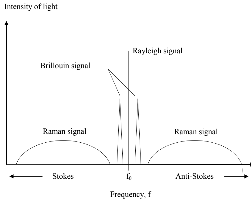
Figure 5 The positions of Rayleigh, Brillouin and Raman scattered light relative to the incident light beam of frequency, f_0 [3]. (Note that these axes are not to scale.)
