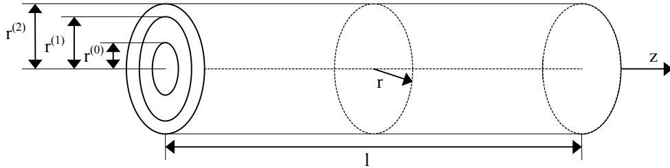
Figure A 1 The geometry of the multi-layered cylinder representation of a jacketed optic fibre.
