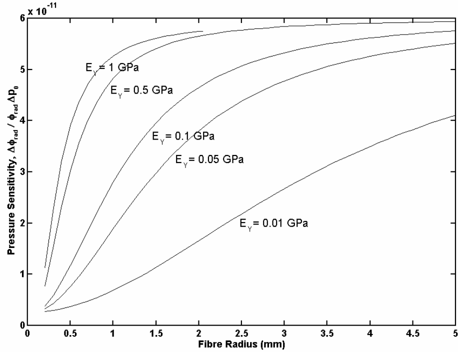
Figure 7 Calculated pressure sensitivity as a function of fibre radius. The different curves are for outer jacket layers with different Young's moduli, E_Y . The bulk modulus, K_b , was kept the same (4 GPa) in each case.
