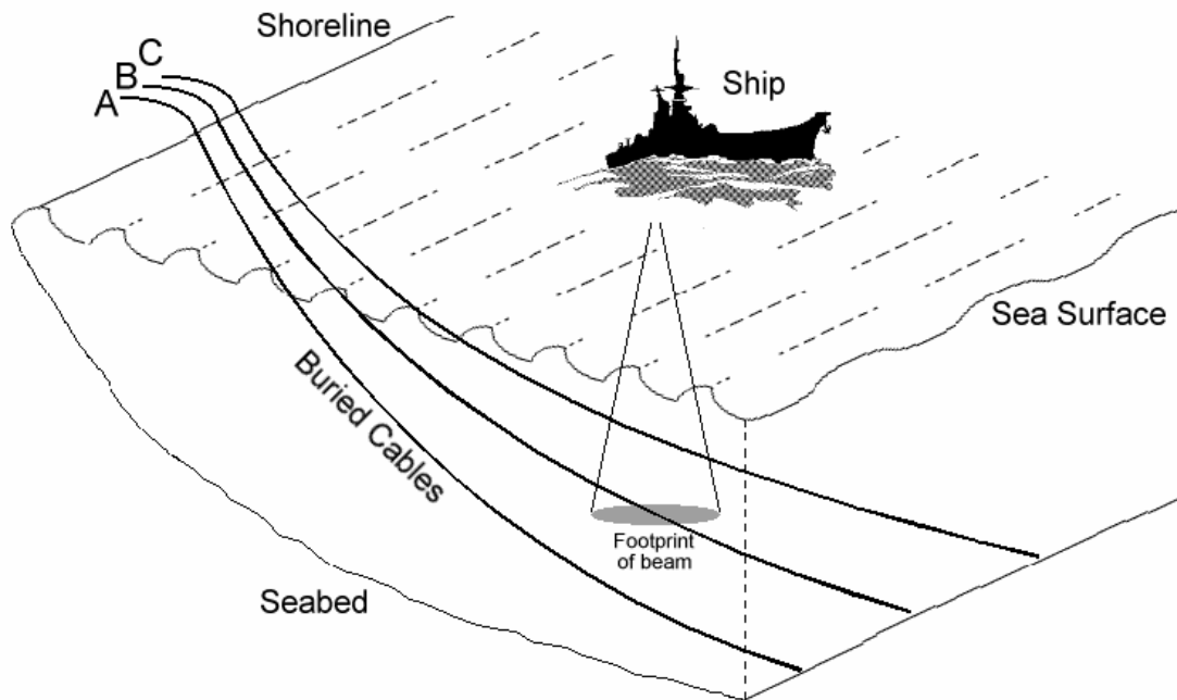
Figure 1 The detection protocol associated with an acousto-optic detection system. In this scenario, an acoustic beam is projected from a surface vessel (though it could also be projected from an ROV). As the footprint of the beam passes over cable B, its affect on the optical transmission properties of the inner fibres may be detected using a land-based system. By comparing the position of the footprint over time with the time of detection, it should be possible to determine the location of the cable.
