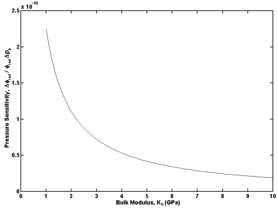
Figure 8 Calculated pressure sensitivity as a function of bulk modulus, K_b , for a large radius (3 mm) outer jacket. Young's modulus, E_Y , was kept constant (0.1 GPa).
