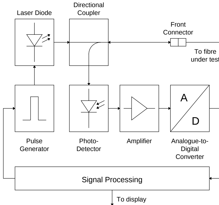
Figure 2 The architecture of an optical time-domain reflectometry system.
