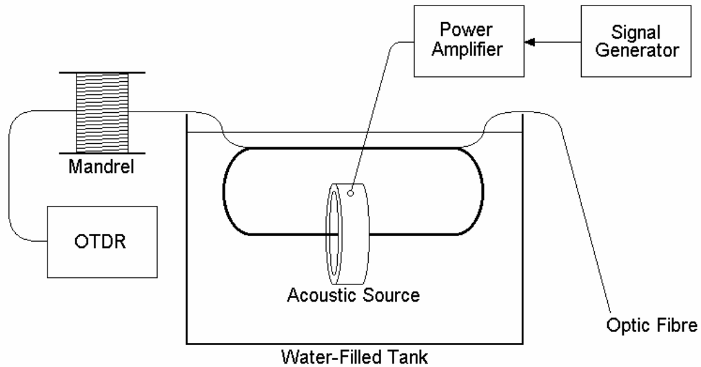
Figure 9 The apparatus used in the OTDR experiment. The OTDR was connected to a 1.8 km length of optic fibre wound on a mandrel. The final 8 m of fibre was wound through a submerged tubular acoustic source. The fibre was excited using the acoustic source, and the back-scattered optical signal was measured using the OTDR.
