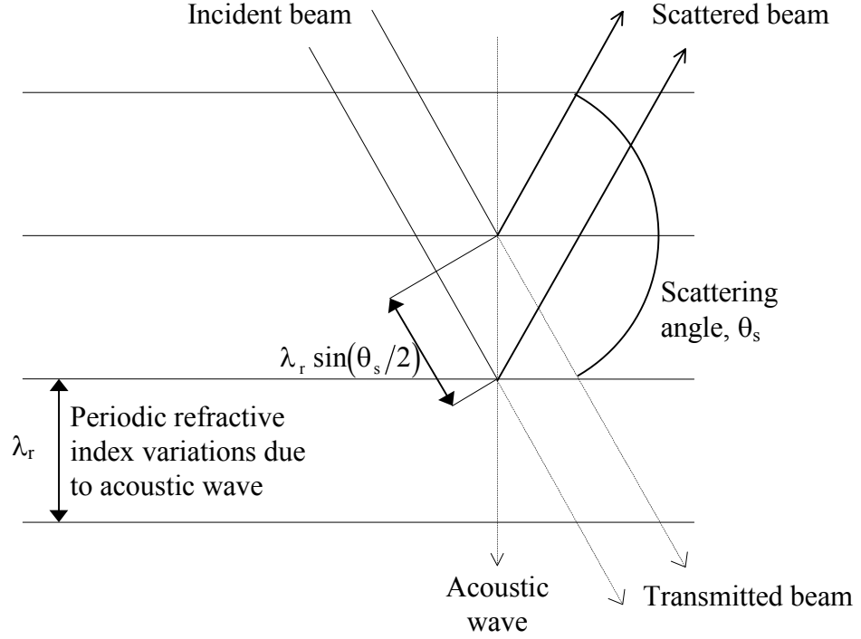
Figure 6 Bragg scattering from periodic refractive index variations in an otherwise homogeneous medium. The scattered beam will only be coherent if the path length, 2\lambda_r \sin(\theta_s/2) , is an integer multiple of the wavelength of the incident beam, \lambda_p/n_r .
