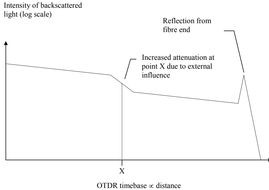
Figure 3 The OTDR output trace. The intensity of the back-scattered signal is displayed as a function of time (proportional to fibre length). An almost constant attenuation is observed over the length of the fibre except at point X where some external influence has caused the attenuation to increase.
