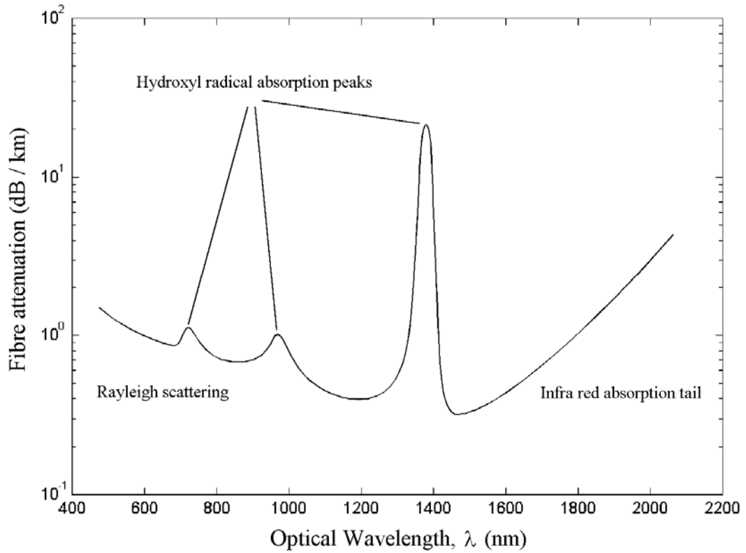
Figure 4 The characteristic optical attenuation spectrum of glass optic fibres [10].
