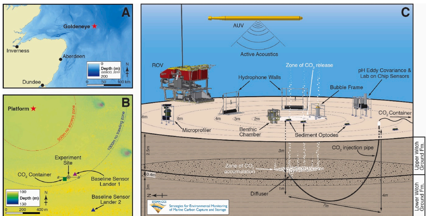
Fig. 1. Location and experimental geometry of the controlled CO 2 release experiment in the North Sea at 120 m water depth. A , Regional map showing the location of the Goldeneye Platform (red star), ~130 km NE of Aberdeen. B , Location of the controlled release experiment site SE of the Goldeneye Platform, seabed CO 2 container (~80 m SW of the experiment site), Baseline Sensor Landers. Chirp sub-bottom profile transect (a-a'; Fig. 3). C , Detailed experimental geometry around the locus of the release showing seabed instrumentation deployed by a Remotely Operated Vehicle (ROV). The CO 2 release was 3 m below the sediment surface immediately below a 30–50 cm thick sandy layer (stippling) at the top of the Lower Witch Ground formation. The rest of the Lower Witch Ground formation (~3 m) and the overlying Upper Witch Ground formation (~2.5 m) comprise moderately sorted sandy and silty muds.
