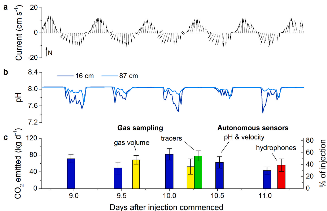
Fig. 6. Detection and quantification of total \text{CO}_2 emitted from the seafloor at the highest release rate. a , Direction and magnitude of tidal currents, which drive the \text{CO}_2 -enriched water towards the chemical sensors during south-bound flow. b , pH of the water at 16 and 87 cm above the seafloor, 2.6 m south of the release point. c , estimates of the total flow rate of \text{CO}_2 emitted from the seafloor in \text{kg day}^{-1} (left y-axis) and as a fraction of actual \text{CO}_2 injection (right y-axis). These estimates are determined from: physical measurement of bubble flow rate using funnels of the gas bubble samplers (“gas volume”); analysis of tracer concentration in gaseous samples collected \sim 15 cm above the seafloor (“tracers”); passive acoustics measuring sound of bubble ebullition (“hydrophones”); and lab-on-chip pH measurements coupled with velocity data and models of bubble dissolution and hydrodynamics (“pH & velocity”). The first three techniques estimate gaseous \text{CO}_2 emission from seafloor while the last one estimates the total \text{CO}_2 in the plume after complete dissolution.
