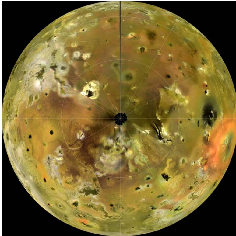
Figure 1. Io is the most volcanically active body in the Solar System. Volcanoes erupt massive volumes of silicate lava, sulphur and sulphur dioxide, constantly changing Io's appearance. Images have been produced by combining the best images from both the Voyager 1 and Galileo Missions. This image shows the South Polar regions of Io. The massive red deposit around Pele is the most distinctive expression of volcanic activity on Io. This image is provided courtesy of NASA/JPL (original in colour), and the caption is based on text supplied by NASA.
