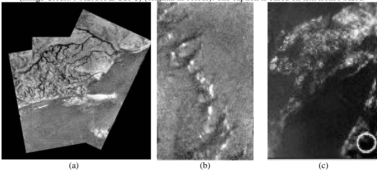
Figure 7. Images of Titan obtained by the Huygens probe. (a) This mosaic of three frames provides detail of a high ridge area including the flow down into a major river channel from different sources. (b) A single image from the Huygens DISR instrument of a dark plain area on Titan, seen during descent to the landing site. There appears to be flow around bright 'islands'. The areas below and above the bright islands may be at different elevations. (c) The landing site of Huygens is circled. (Credits: ESA/NASA/JPL/University of Arizona). The caption is based on text from NASA.
