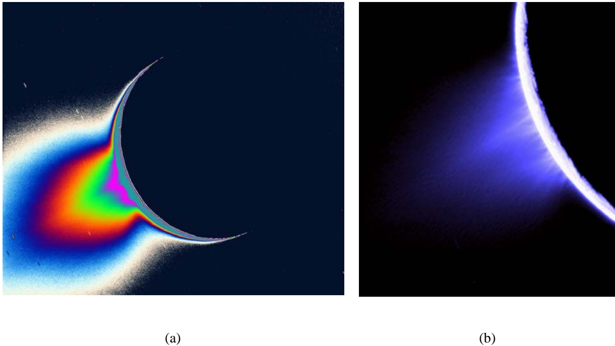
Figure 2. (a) Cassini images of Saturn's moon Enceladus backlit by the sun show the fountain-like sources of the fine spray of material that towers over the south polar region. The image was taken using the Imaging Science Subsystem (Narrow Angle), looking more or less broadside at "tiger stripe" fractures Enceladus images. It shows discrete plumes of a variety of apparent sizes above the limb of the moon. The greatly enhanced and colorized image shows the enormous extent of the fainter, larger-scale component of the plume. Imaging scientists, as reported in the journal Science on March 10, 2006, believe that the jets are geysers erupting from pressurized subsurface reservoirs of liquid water above 273 degrees Kelvin (0 degrees Celsius). (b) Cassini imaging scientists used views like this one to help them identify the source locations for individual jets spurting ice particles, water vapour and trace organic compounds from the surface of Saturn's moon Enceladus. Their study -- published in the Oct. 11, 2007, issue of the journal Nature -- identifies eight source locations, all on the prominent tiger stripe fractures, or sulci, in the moon's south polar region. Some of the sources occur in regions not yet observed by Cassini's composite infrared spectrometer, and the researchers predict that future Cassini observations of those locations will find elevated temperatures. This false-colour view was created by combining three clear filter images taken at nearly the same time as the image shown in (a). This image product was then specially processed to enhance the individual jets that compose the plume (the image shown in (a) was instead processed to reveal subtleties in the brightness of the overall plume that comprises the jets). Some artefacts due to the processing are present in the image. The final product was coloured as blue for dramatic effect. The images were acquired with the Cassini spacecraft narrow-angle camera on Nov. 27, 2005 at a distance of approximately 148,000 kilometers (92,000 miles) from Enceladus and at a sun-Enceladus-spacecraft, or phase, angle of 161 degrees. Scale in the original images is about 880 meters (0.5 mile) per pixel. This view has been magnified by a factor of two from the original images. These images were provided courtesy of NASA/JPL (original in colour) and the caption is based on text from NASA.
