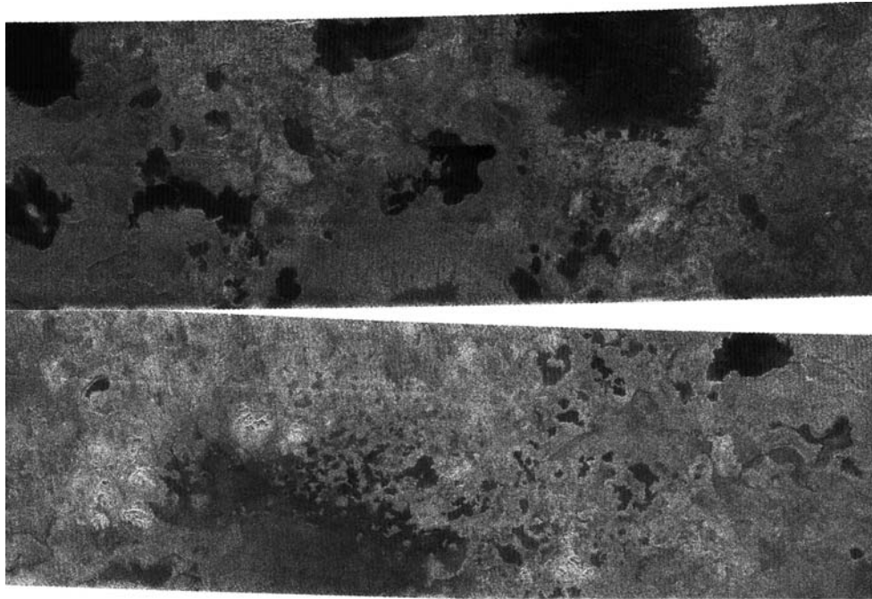
Figure 8. These two radar images were acquired by the Cassini radar instrument in synthetic aperture mode on July 21, 2006. The top image centred near 80 degrees north, 92 degrees west measures about 420 km by 150 km (260 miles by 93 miles). The lower image centred near 78 degrees north, 18 degrees west measures about 475 km by 150 km (295 miles by 93 miles). Smallest details in this image are about 500 meters (1,640 feet) across. The variety of dark patches in the image suggests the presence of many lakes in the high latitudes around the North Pole of Titan. Some of these dark patches have channels leading in or out of them. The channels have a shape that strongly implies they were carved by liquid. Some of the dark patches and connecting channels are completely black, that is, they reflect back essentially no radar signal, and hence must be extremely smooth. In some cases rims can be seen around the dark patches, suggesting deposits that might form as liquid evaporates. Because such lakes may wax and wane over time, and winds may alter the roughness of their surfaces, repeat coverage of these areas should test whether these are indeed bodies of liquid. (Image Credit: NASA/JPL). The caption is based on text from NASA.
