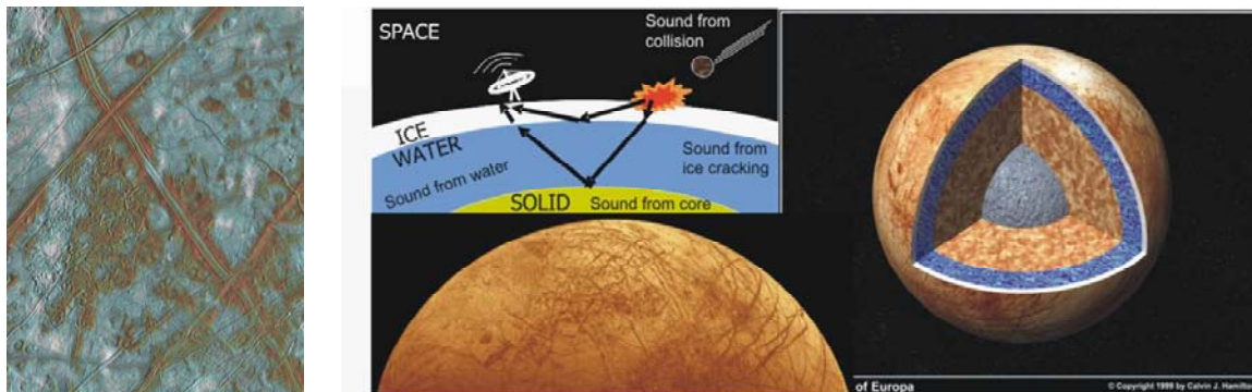
Figure 4. (a) Cracks on Europa's ice surface. Most scientists believe that salts and other inorganic materials are responsible for the coloured patches on Europa's outer layer, although there has been speculation that bacteria, extruded through the ice from below and 'flash frozen' on the surface, are responsible. (Credit: NASA/JPL) (b) Top left: schematic of possible acoustic-based mission to Europa, where acoustic signals originating from various planetary sources are passively detected and transmitted to Earth via an orbiter: ray paths and scales are for illustrative purposes only (schematic from reference [55]). Lower: the surface of Europa, showing ice features (Credit: NASA/JPL). Right: Schematic of the interior of Europa showing ice covering over a water ocean, overlaying the solid interior (Copyright Calvin J Hamilton). (Original in colour).
