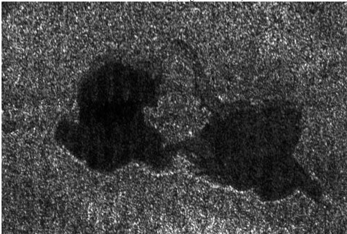
Figure 5. In this Cassini radar image, two of Titan's lakes (near 73 degrees north latitude, 46 degrees west longitude) are seen, each 20 to 25 kilometers (12 to 16 miles) across. The image from a flyby on Sept. 23, 2006, covers an area about 60 kilometers (37 miles) wide by 40 kilometers (25 miles) high. They are joined by a relatively narrow channel. The lake on the right has lighter patches within it, indicating that it may be slowly drying out as the northern summer approaches. This image is provided courtesy of NASA/JPL and the caption is based on text from NASA.
