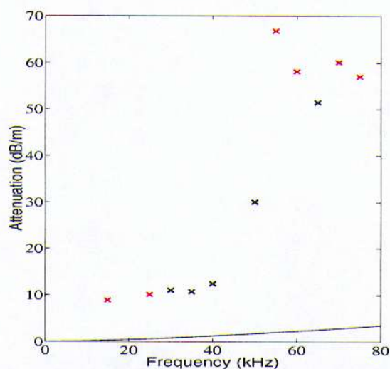
Figure 7. Frequency dependent attenuation: measured attenuations based on three or more amplitudes (X) and two amplitudes (X) and fast wave attenuation predicted by the Biot model (black line). Errors are omitted as they are less than 0.1 dB/m.
