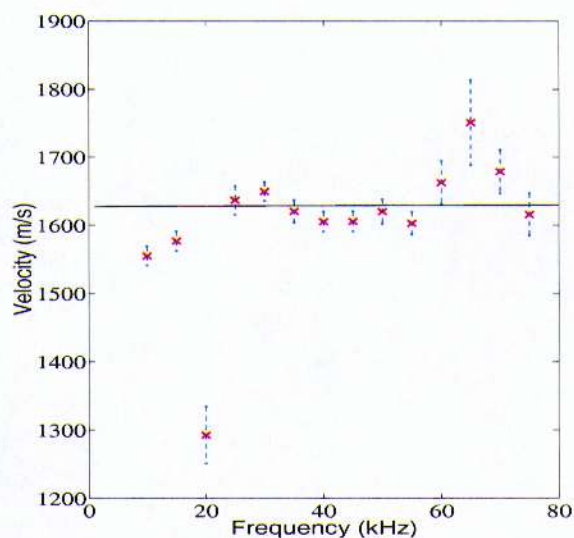
Figure 5. Frequency dependent velocity: measured velocities (X), with errors corresponding to 95% confidence limits, and fast wave velocity predicted by Biot model (black line).
