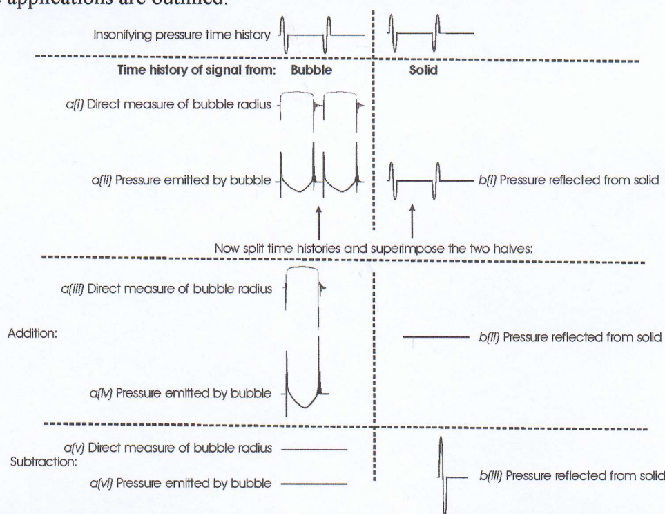
FIGURE 5. Schematic of a proposed 'Twin Inverted Pulse Sonar', whereby the scattering from a linear scatterer (such as a solid, a mine, or a swim bladder insonified at frequencies much greater than its resonance), and scattering from nonlinear scatterers (such as bubbles) can be enhanced and suppressed relative to one another (see text). The schematic bubble radius and time histories are justified in [7].
