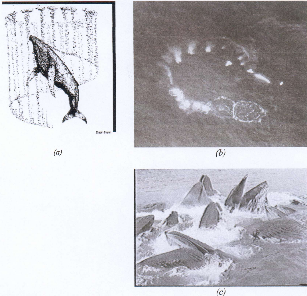
FIGURE 1. (a) Schematic of a humpback whale creating a bubble net. A whale dives beneath a shoal of prey and slowly begins to spiral upwards, blowing bubbles as it does so, creating a hollow-cored cylindrical bubble net. The prey tend to congregate in the center of the cylinder, which is relatively free of bubbles. Then the whale dives beneath the shoal, and swims up through the bubble-net with its mouth open to consume the prey ('lunge feeding'). Groups of whales may do this co-operatively (Image courtesy of Cetacea.org). (b) Aerial view of a humpback bubble net (photograph by A. Brayton, reproduced from [10]). (c) Humpback whales lunge feeding (Image courtesy of L. Walker, http://www.groovedwhale.com ).
