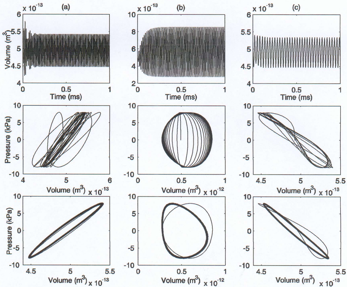
FIGURE 4. Bubble responses for a 49 \mu\text{m} bubble insonified by a semi-infinite pulse starting at t=0 with an amplitude of 7.95 \text{ kPa} at (a) 84.2 \text{ kHz} (b) 65.7 \text{ kHz} and (c) 31.5 \text{ kHz} . The top graph in each case shows the volume time history calculated using the Keller-Miksis equation (with damping after [32]). The middle graph in each case shows the corresponding pressure-volume curve. The darker area in each PV curve shows the steady state regime, where the successive loci overlap each other. Nonlinear components will cause crossovers in a loop (as in Fig. 4c where a second harmonic arises from driving the bubble close to half resonance frequency), such that the integration of (12) causes the areas of the clockwise loops to be subtracted from those of the anticlockwise. The bottom row superimposes the steady-state loops of the middle row (thin line) with the corresponding linear solution using the steady-state formulation of Commander and Prosperetti [1] (thick line). Figure by T. G. Leighton, S. D. Meers, and P. R. White [2].
