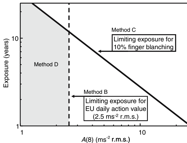
Fig. 1 Limiting exposures for Method B (EU daily exposure action value of 2.5 \text{ m s}^{-2} \text{ r.m.s.} ), Method C (exposures corresponding to 10% prevalence of vibration-induced white finger according to ISO 5349, 2001), and Method D (combination of Methods B and C—shown in grey)
