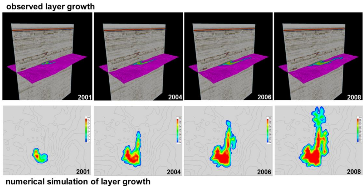
Figure 3.11 History-matching the topmost layer of CO 2 in the Sleipner plume. Upper boxes show 3D views of the top reservoir surface (purple) and the observed topmost CO 2 layer reflectivity (colours). The lower boxes show maps of the modelled topmost layer (bottom). The top reservoir surface in the 3D views covers an area of around 3 x 7 km. Seismic data courtesy of Statoil ASA. (British Geological Survey © NERC 2014).
