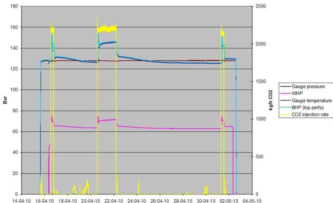
Figure 3.23 Plot of pressures, temperatures and flow at well K12-B6. (Courtesy of Vandeweyer et al., 2011 and TNO contribution to the CO2ReMoVe project).
