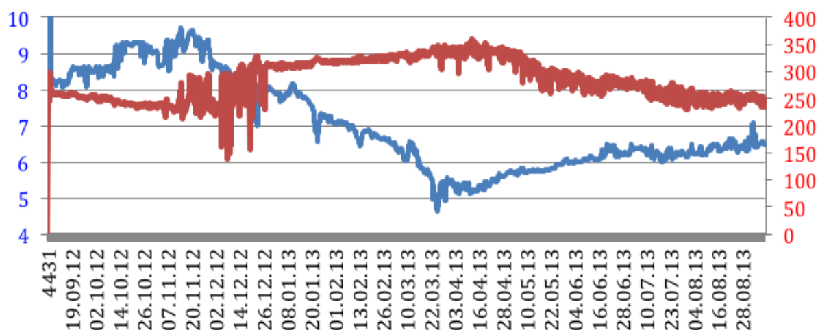
Figure 4.8 Raw data from an Aanderaa Recording Current Meter (RCM) deployed on a seabed lander September 2012- October 2013. Blue temperature (°C) and red oxygen concentration (µM). (Data courtesy ECO2 project and copyright National Oceanography Centre, NERC).
