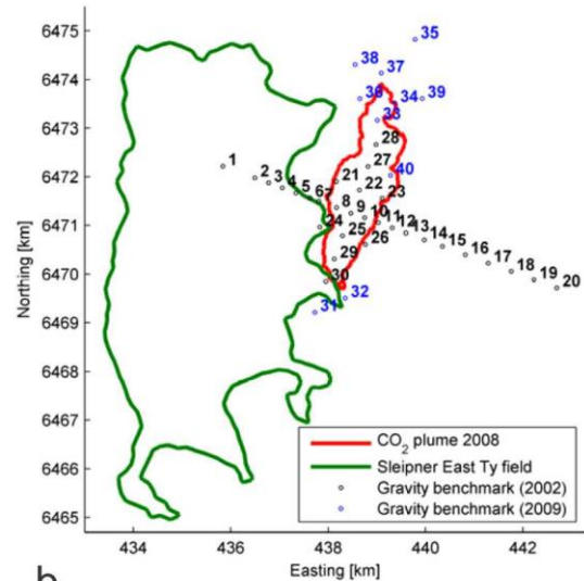
Figure 3.18 a) ROV and seabed gravimeter deployed at Sleipner b) location of the gravimetry benchmarks with respect to the 2008 CO 2 plume footprint (courtesy of Statoil ASA).
