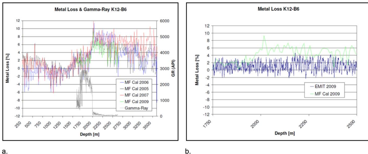
Figure 3.24 Time-lapse well integrity studies in the K12-B injection well. Left: Multi-finger caliper (MF Cal) calculated metal loss results and gamma ray. Right: Detail of electromagnetic imaging (EMIT) and multi-finger (MF) caliper calculated metal loss (Vandeweijer V.P. and Arts R personal communication).
