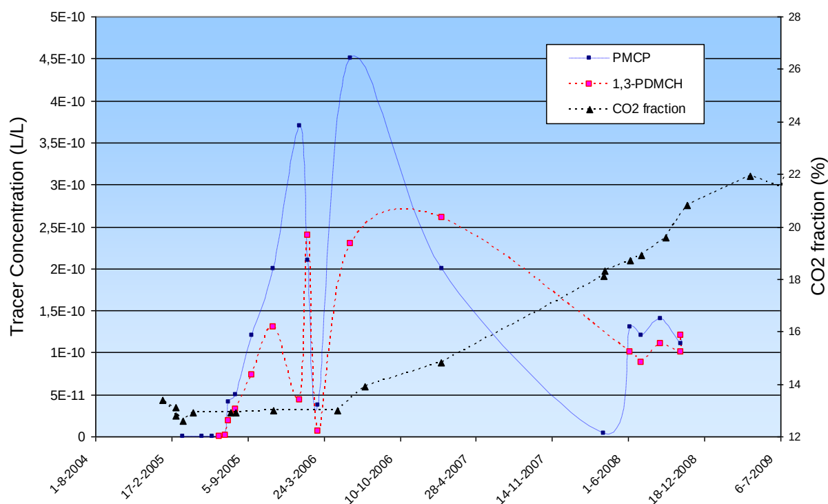
Figure 3.26 Tracer concentrations and CO 2 concentration at the K12-B1 production well. (420 m from the injector well) (after Vandeweyer et al., 2011b).
