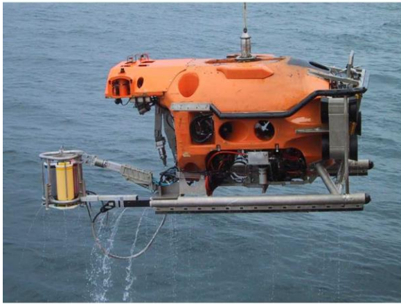
Figure 3.18 a) ROV and seabed gravimeter deployed at Sleipner b) location of the gravimetry benchmarks with respect to the 2008 CO 2 plume footprint (courtesy of Statoil ASA).
